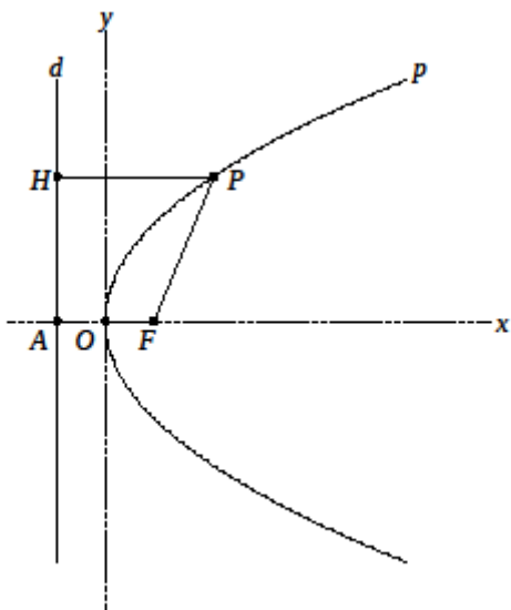
Fig. 1 Focus and directrix of parabola
