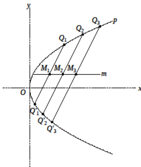
Fig. 2 Diameter of parabola
