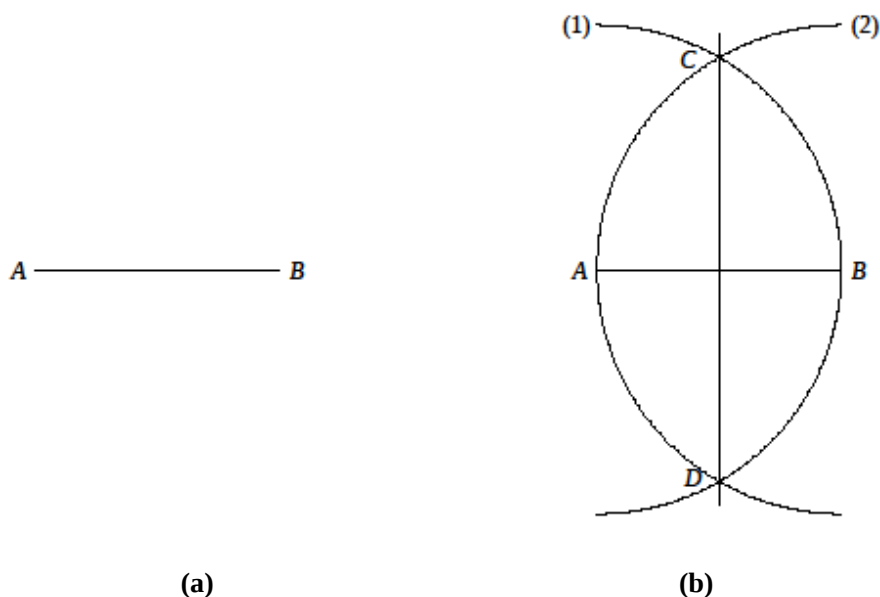
Fig. 3 (a) Line AB, (b) Perpendicular bisector of line AB
